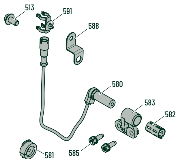
Sensor assembly 05.803.61.73.0 / 74.0
