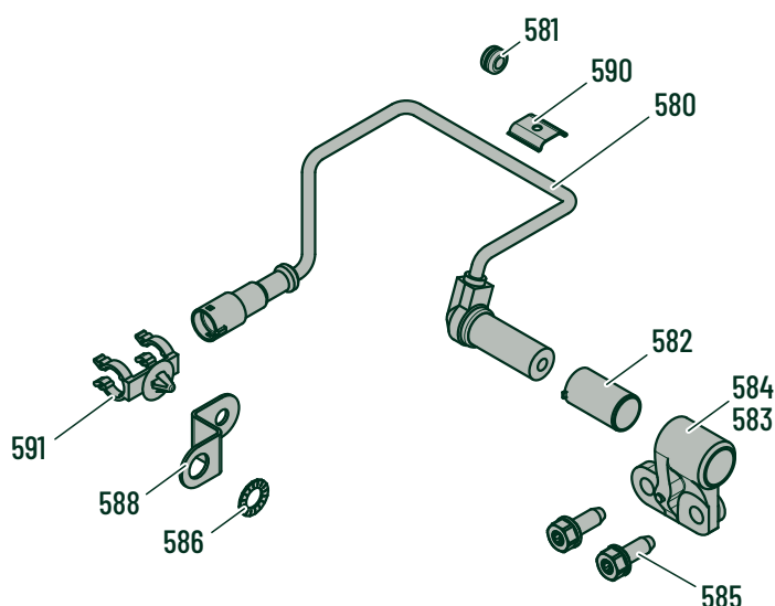
Sensor assembly 05.803.61.73.0 / 74.0
